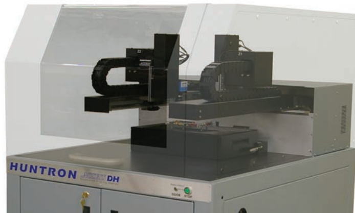
The Access DH provides ample space for large CCAs and assemblies such as CCA fixtures, Interface Test Adapters and more.
