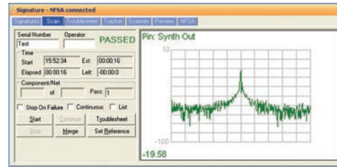
Using the Huntron Workstation SDK, this NFA signature can be displayed in the Workstation Signature pane
